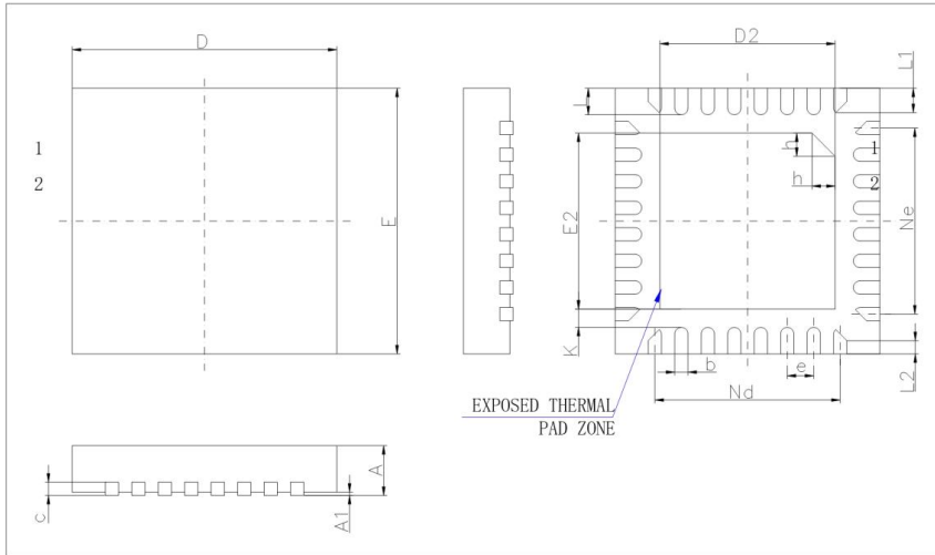
Figure 4-1 AC7106C Package
