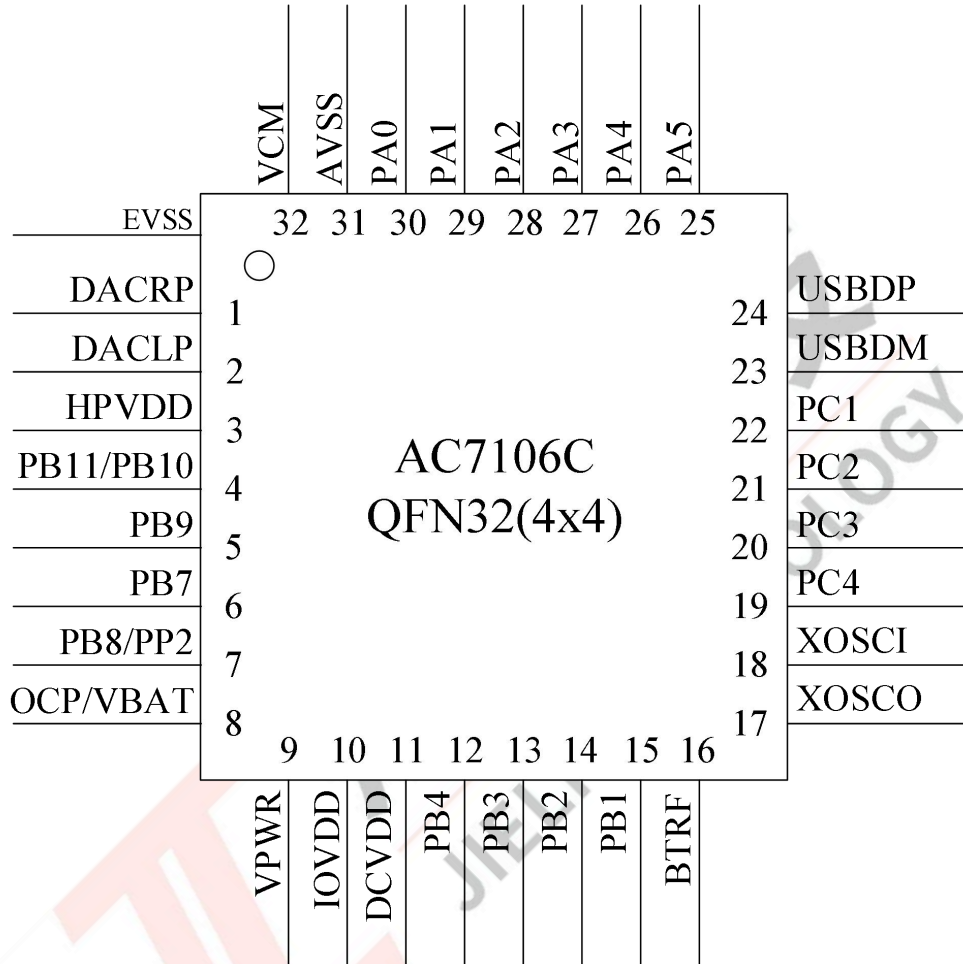
Figure 2-1 AC7106C Pin Assignment
