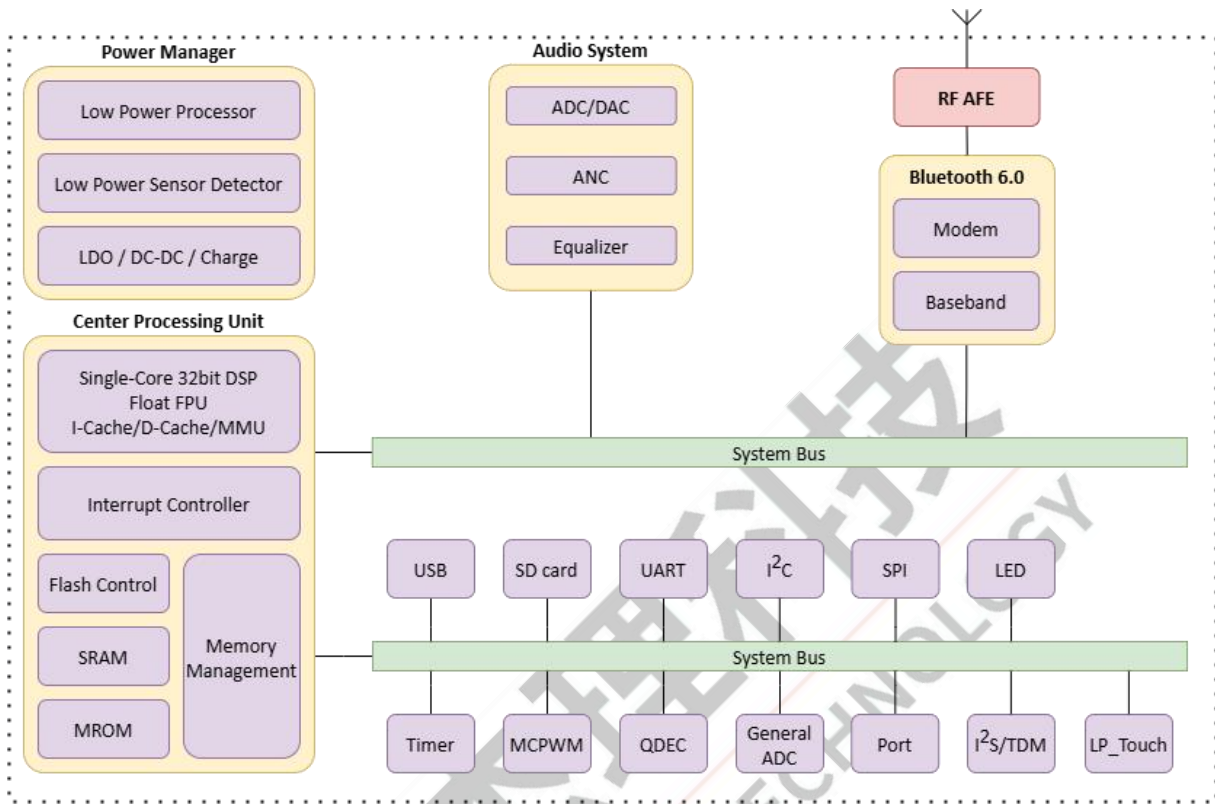
Figure 1-1 AC7106C Block Diagram
