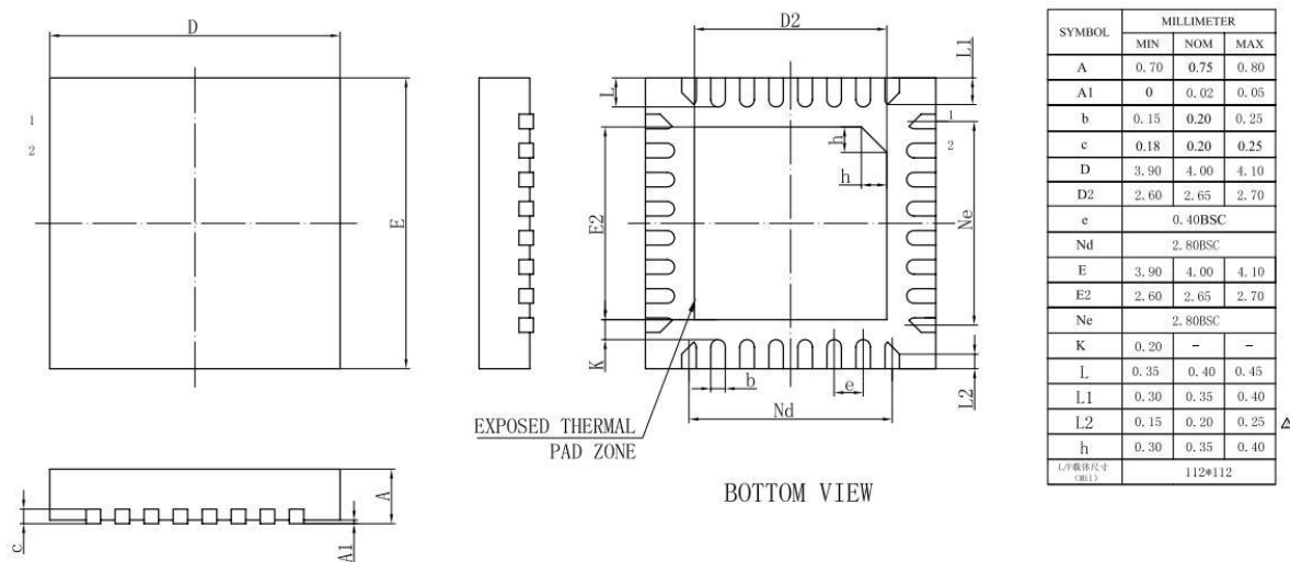
Figure 3-1 AC6956M Package
