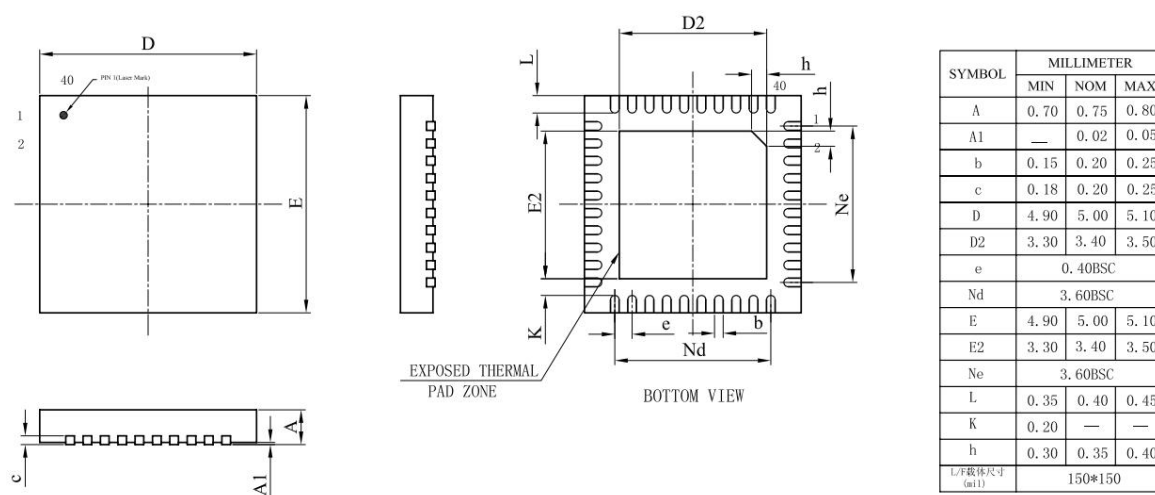
Figure 3-1 AC6958B_QFN40 Package
