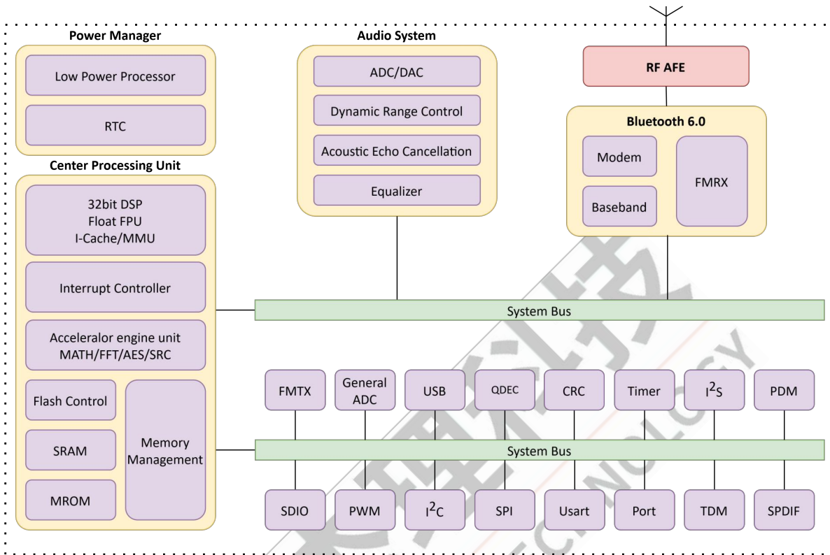
Figure 1-1 AC2106C Block Diagram
