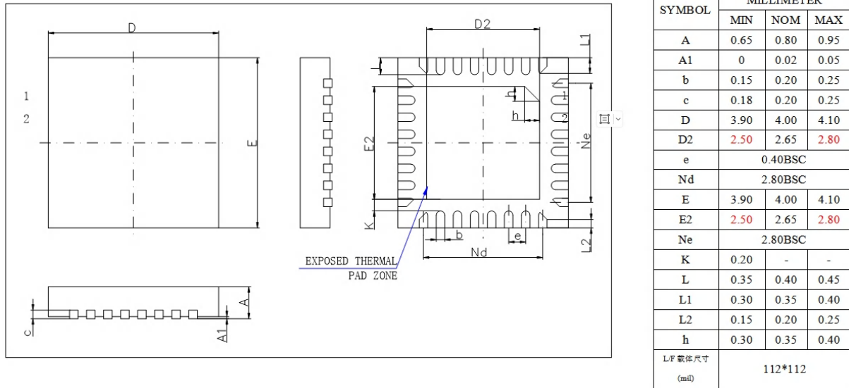
Figure 4-1 AC2106C Package
